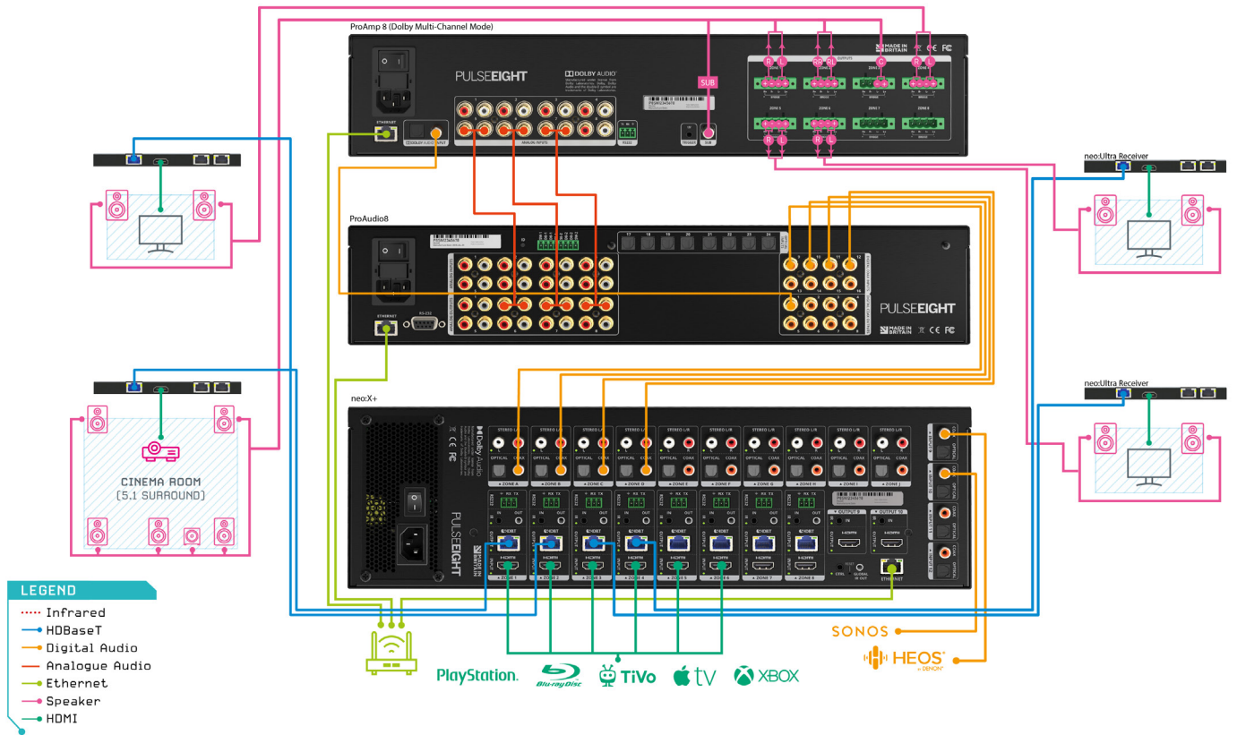
Example of a ProAudio8 wiring with a video matrix (e.g. neoX+) and an amplifier (e.g. ProAmp8).
